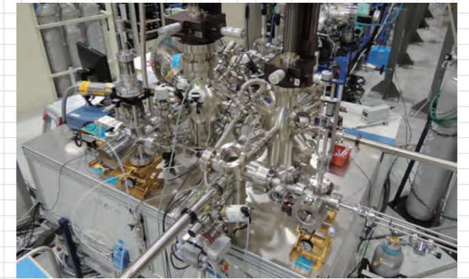
あいちシンクロtron(BL6N1)の放射光XAFS-XPS分析装置 XAFS-XPS analysis system in Aichi SR (BL6N1)
