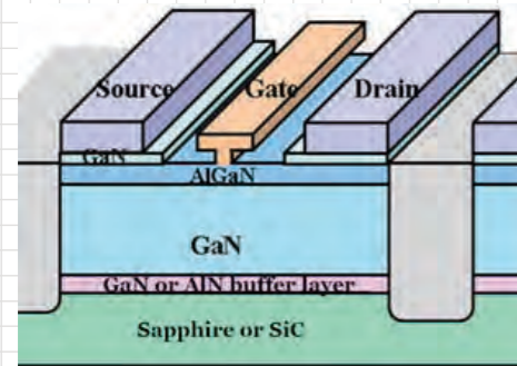
AlGaIn/GaN HEMT
