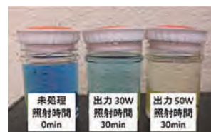
水溶液中染料の超音波分解 Ultrasonic decomposition of dye in aqueous solution
