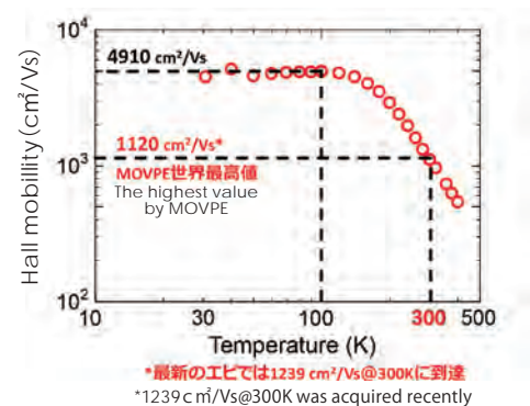
図2. N型低濃度エピのホール移動度 Fig.2 Hall mobility in our n-type low-doping epi-layer
