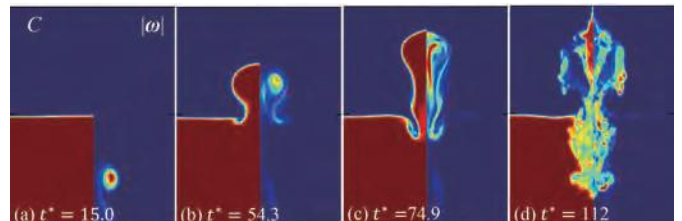
渦輪がもたらす密度成層流体の混合のシミュレーション Simulation of mixing of density-stratified fluid caused by vortex ring
